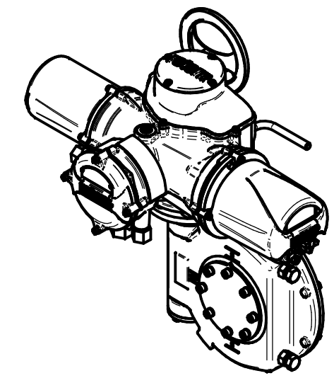
ISOMETRIC VIEW (SCALE 1:12)
