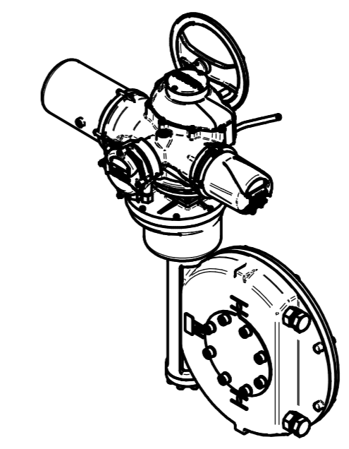
ISOMETRIC VIEW (SCALE 1:20)
