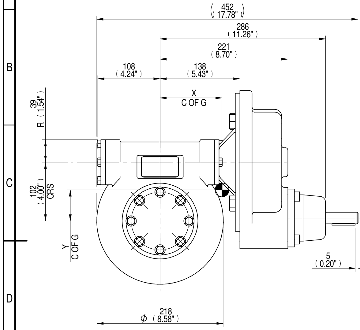
VIEW SHOWING MANUAL OPERATED UNIT
