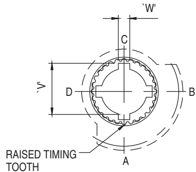
OUTPUT KEYWAY DETAILS SHOWN IN OPEN POSITION
