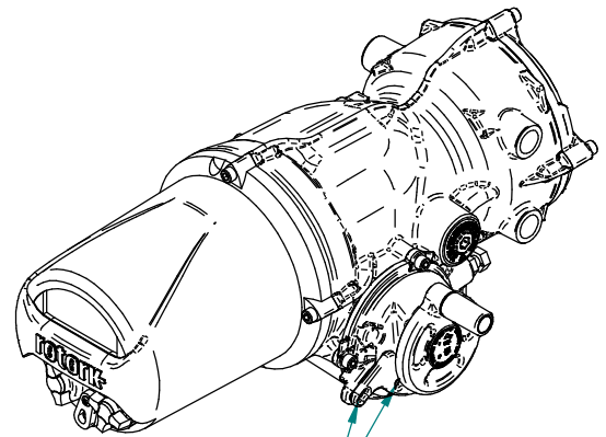
HAND / AUTO LOCKING BOLT HOLES FOR φ8mm HASP PADLOCK
