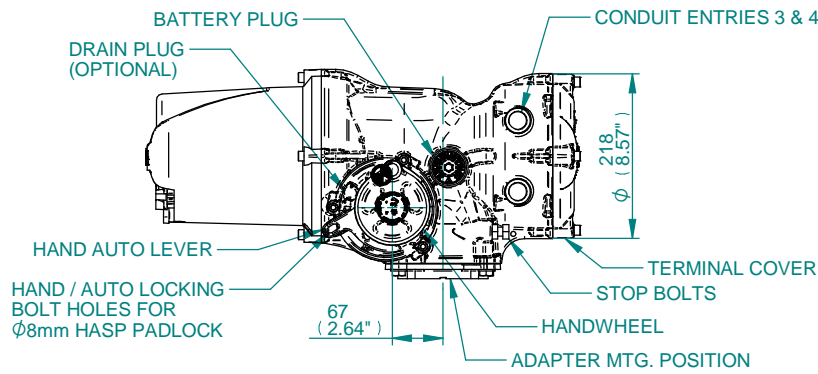
VIEW ON ARROW "A"
