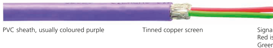
Fig 17: Typical Profibus DP cable specifications
