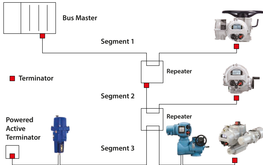
Fig 12: Profibus Single Channel Data Highway Topology
