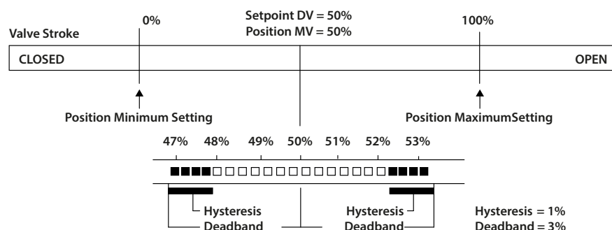
Fig 35: Deadband and Hysteresis settings
