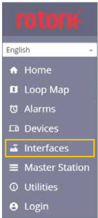
Fig. 6.21 Select Interfaces
