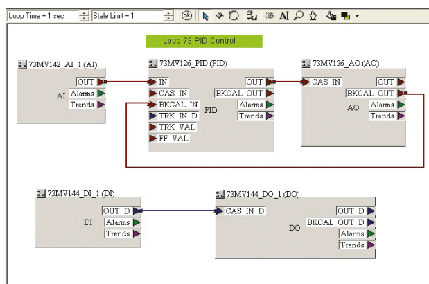
PID Control
