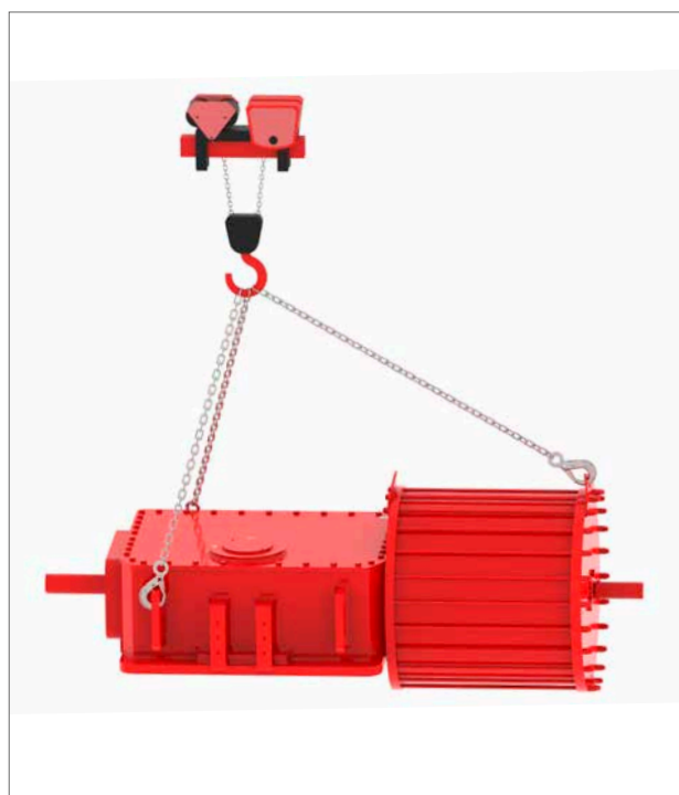
Fig 7.4 Lifting (double-acting actuator size 161-350)
