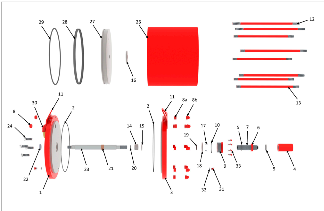
Fig 17.6 Pneumatic cylinder
