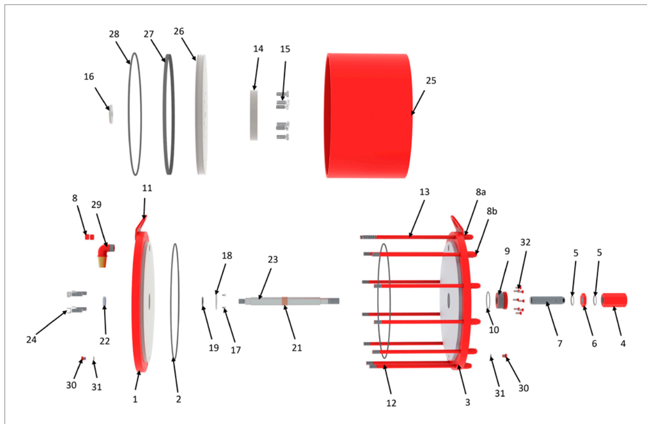
Fig 17.7 Pneumatic cylinder
