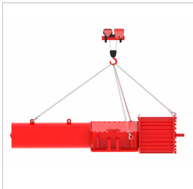
Fig 7.3 Lifting (single-acting actuator size 161-350)
